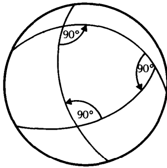
on a sphere a triangle can have three right angles
