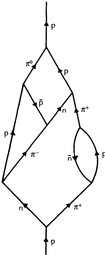
a network of virtual interactions; from Ford, op. cit.
