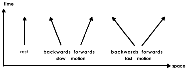
world lines of particles
