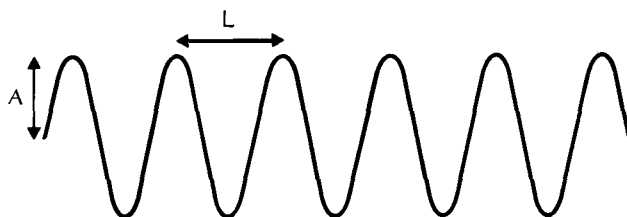
a wave pattern
