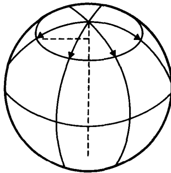
drawing a circle on a sphere
